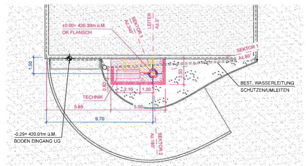
SITUATION 1:200
